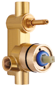
Cat. No. : ST-11 Single Lever Concealed Divertor Body (40mm Cartridge + Tipton Cartridge) MRP. : 4295
